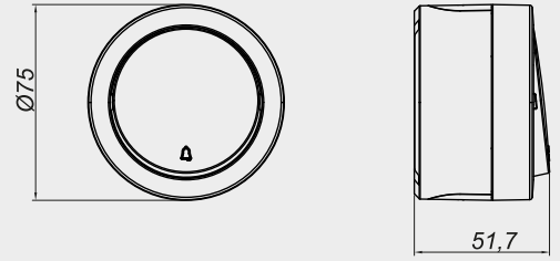
ZİL ANAHTARI
