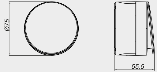
ANAHTAR B.D.
